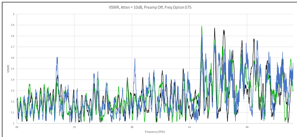
Figure 9. VSWR vs. frequency (26 to 50 GHz), 1a. standard path, 10 dB attenuation, measured on 3 units
