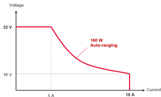
Figure 1. Autoranging technology
