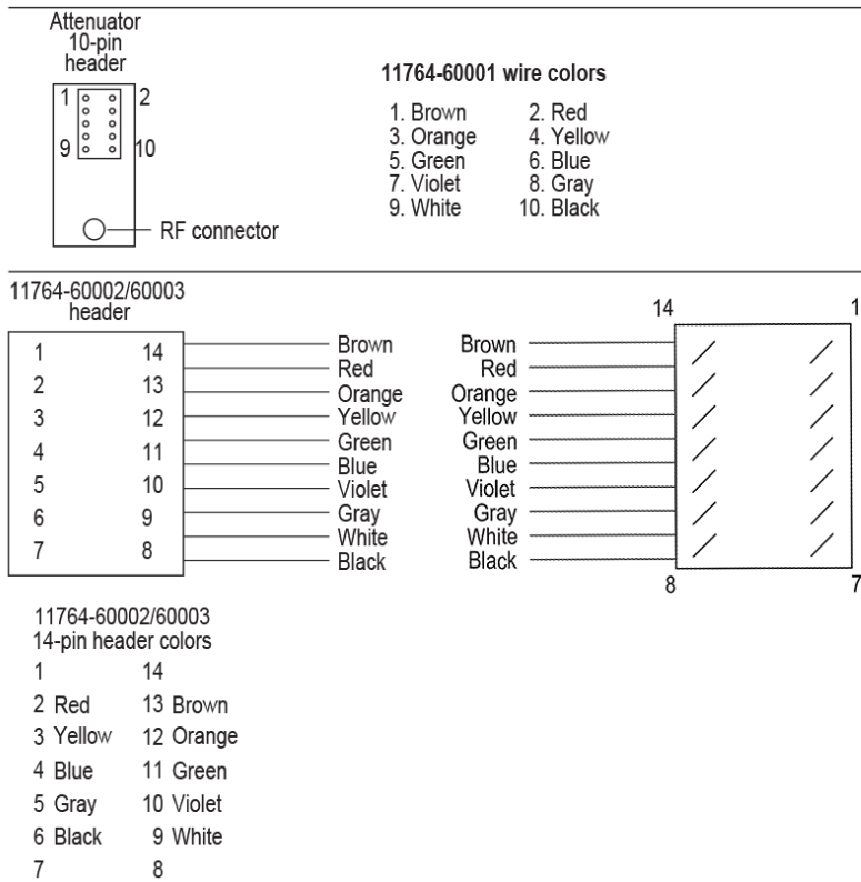
Figure 3. Attenuator switching pinout
