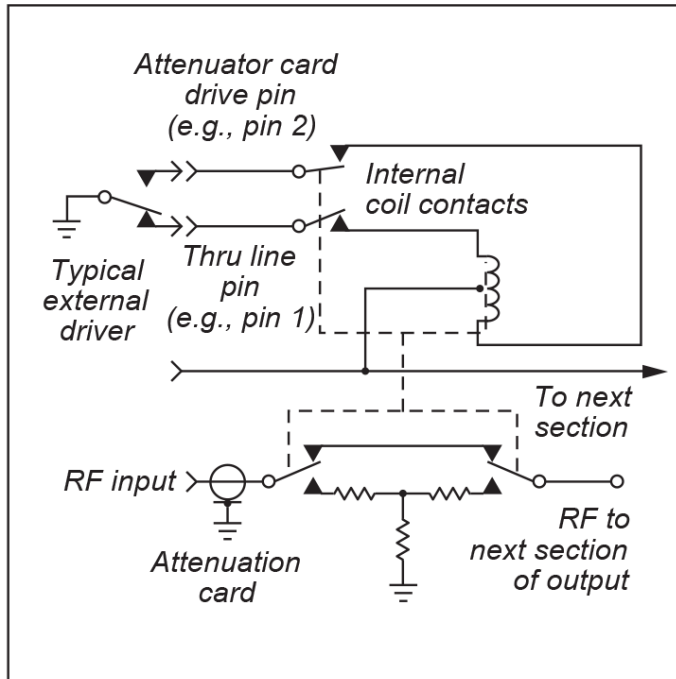
Figure 2. Section electrical diagram
