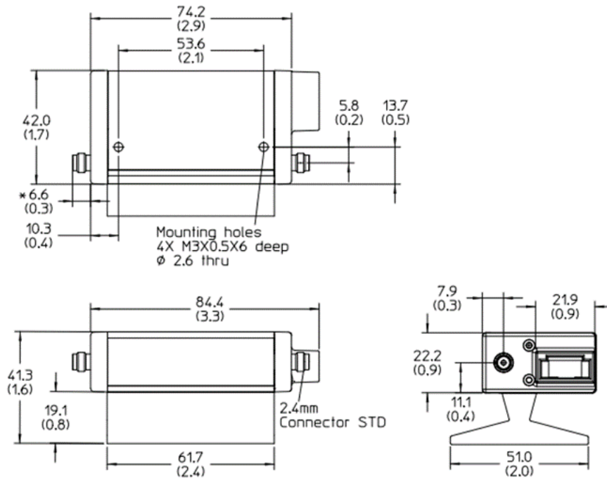
84905M dimensional diagram (dimension are in millimeters and (inches))
