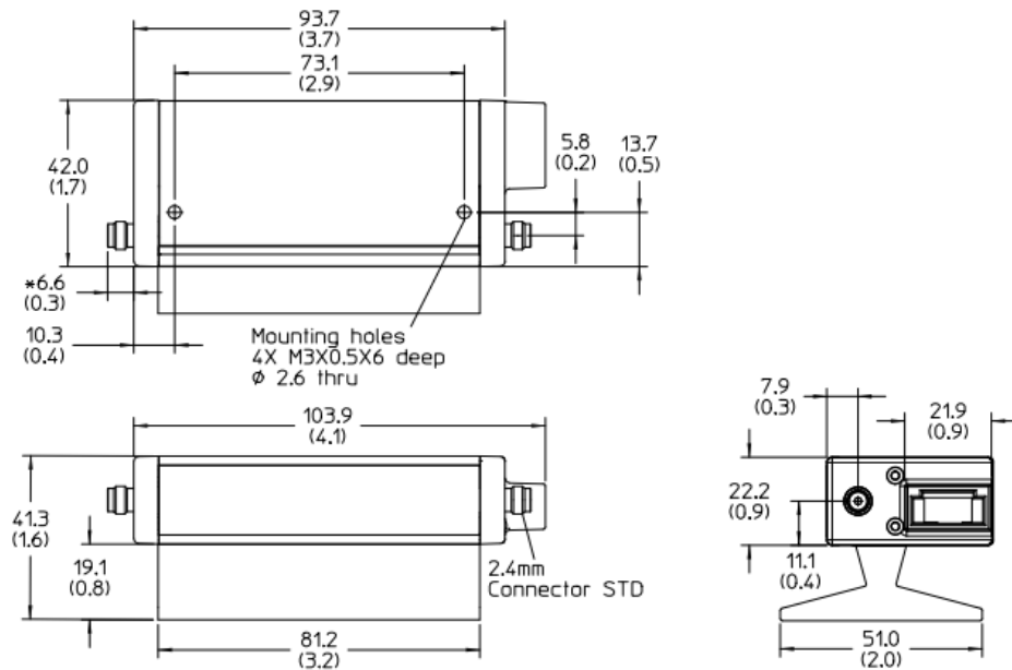
84904/8M dimensional diagram (dimension are in millimeters and (inches))
