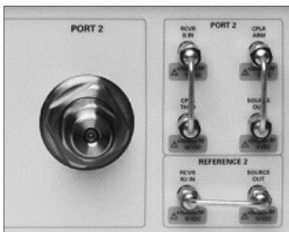
Figure 14. PNA Series front panel: port 2 and jumpers.
