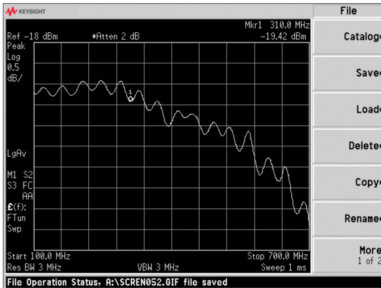
Figure 4. Output-power measurement of a mixer using the configuration illustrated in Figure 1.
