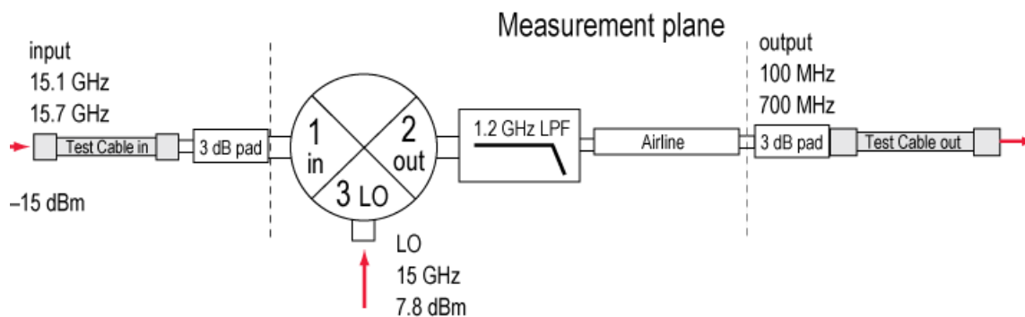
Figure 2. Example of a mixer-under-test with addition of airline.
