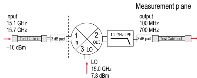
Figure 1. Example of a mixer-under-test configuration.
