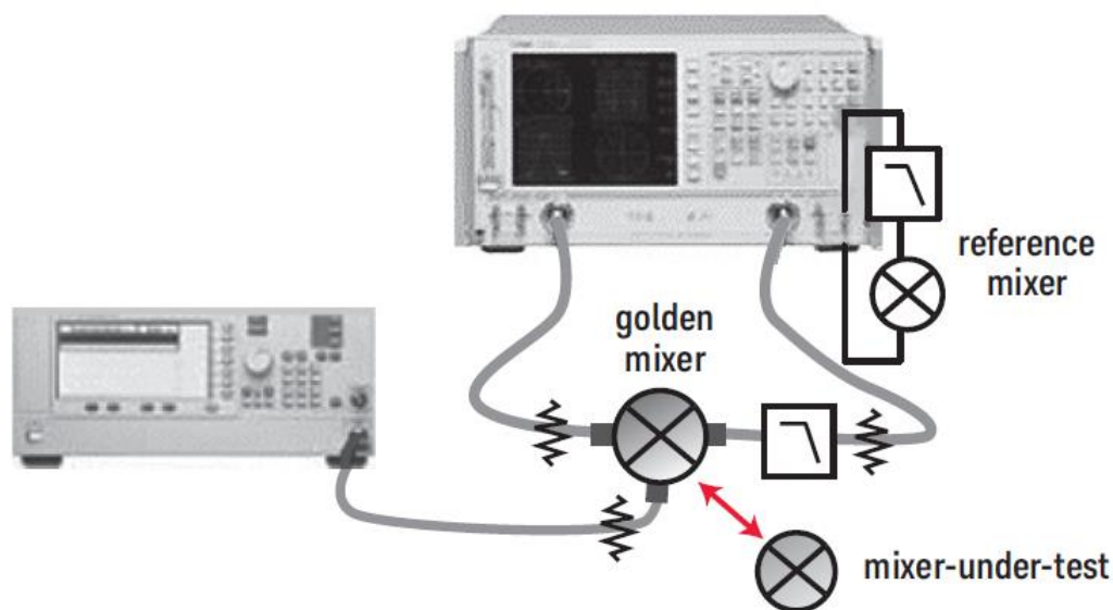
Figure 10. 8720ES group delay configuration using golden and reference mixers.
