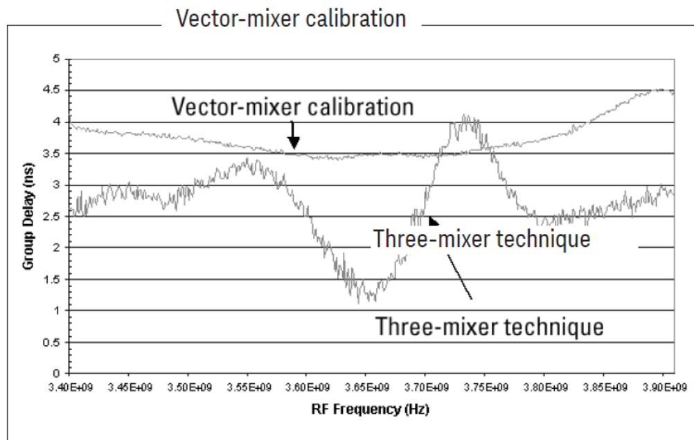
Figure 12. Measurement comparison of group delay techniques.
