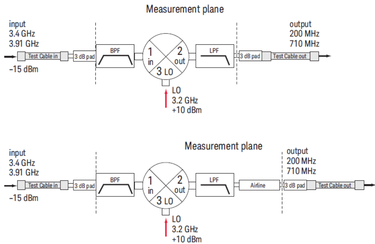
Figure 9. Converter configuration for airline delta comparison.
