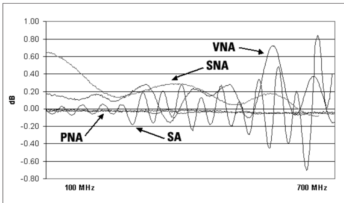
Figure 6. Conversion loss airline delta instrument comparison.
