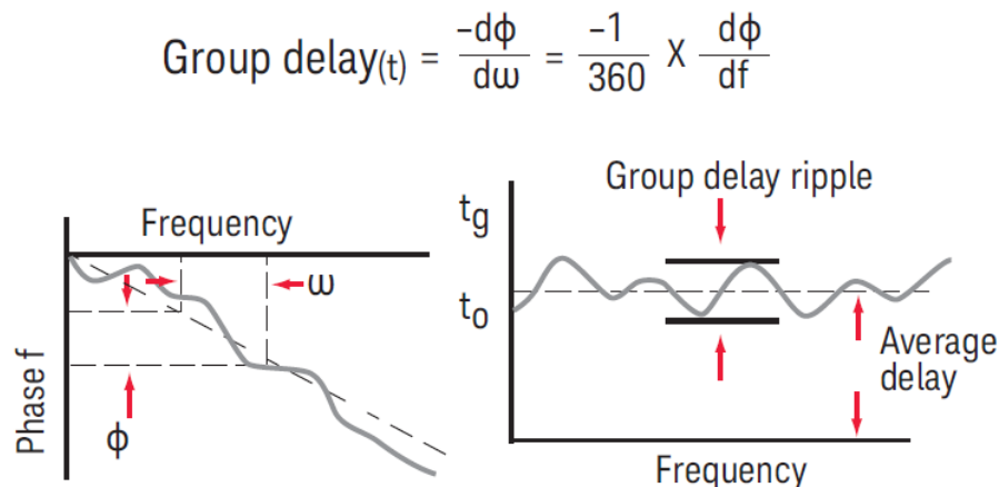
Figure 8. Group delay
