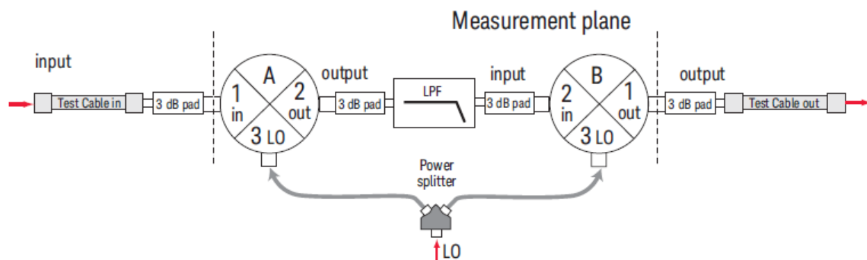
Figure 11. Up/down conversion method measures two mixers in series.
