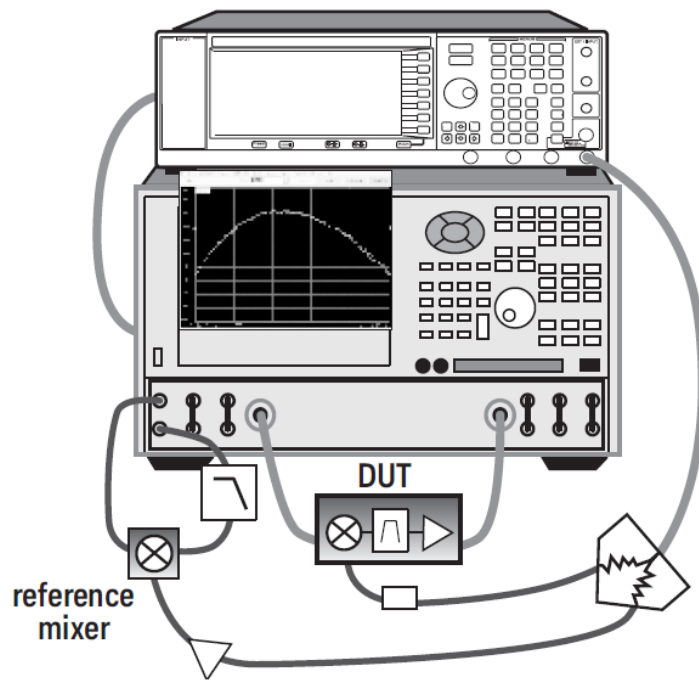
Figure 13. PNA group delay configuration using the vector-mixer calibration.
